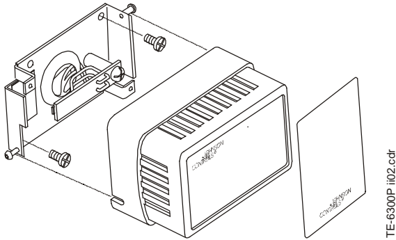
Figure 2: Installing the Wall Mount Sensor
